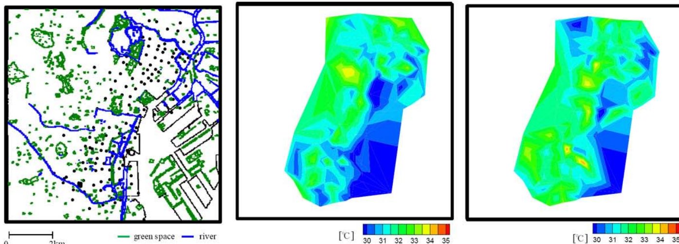
Figure 7. Air temperature distribution at the 173 points of NILIM observation campaign, 1400 LST on 31 July 2005.
